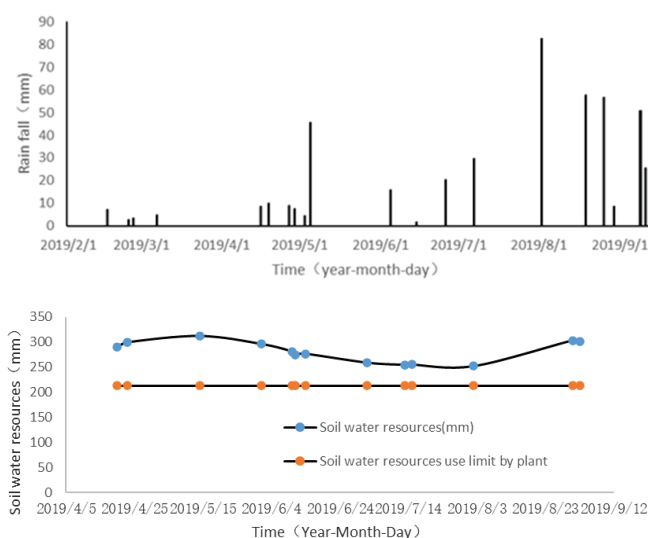
Figure 6: The relationship between Soil Water Resources in the MID and SWRULP in a 2-year-old red plum apricot tree and 24-year-old red plum apricot tree.
