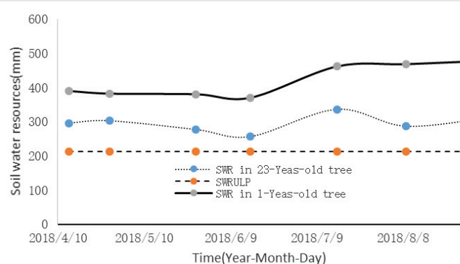
Figure 5: The relationship between soil water resources and the Use Limit of Soil Water Resources by red plum apricot in 1-year-old red plum apricot orchard.
