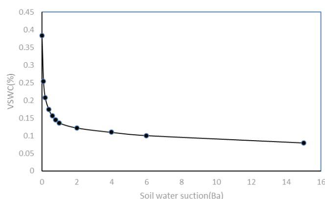
Figure 4: The relationship between the Volume Soil Water Content (VSWC) and soil water suction.
