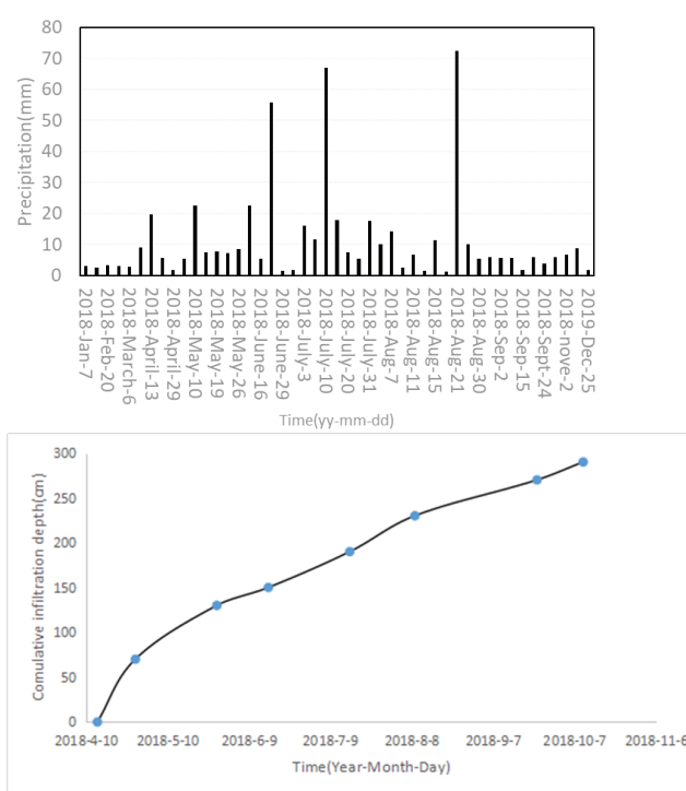
Figure 3: The change of precipitation (top) and soil infiltration depth (bottom) with time in the red plum apricot orchard in 2018.
